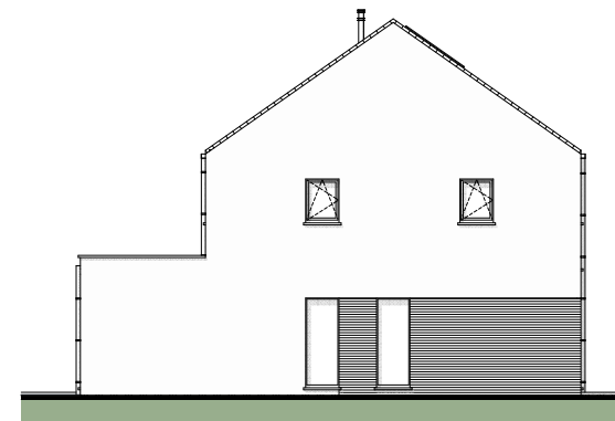
LINKERGEVEL (Lot 2)
